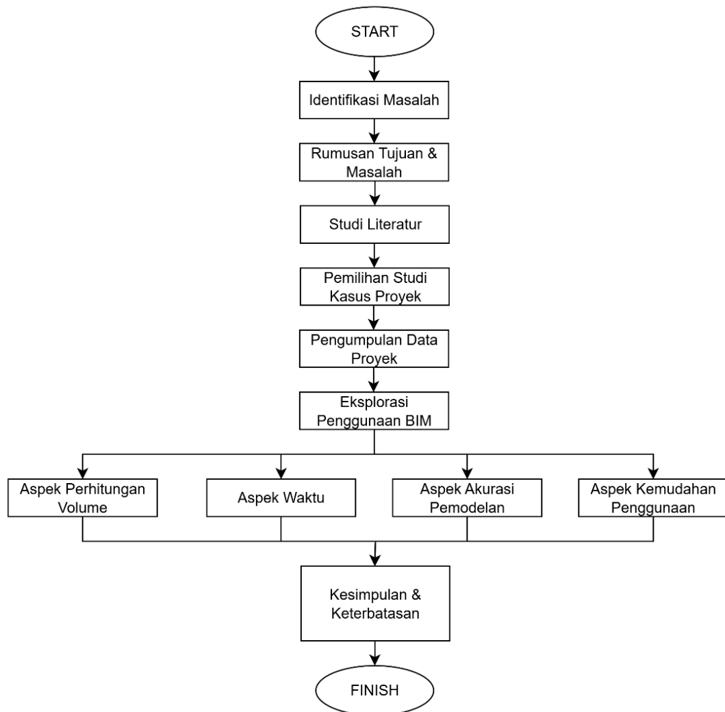
Gambar 1. Flowchart Penelitian
